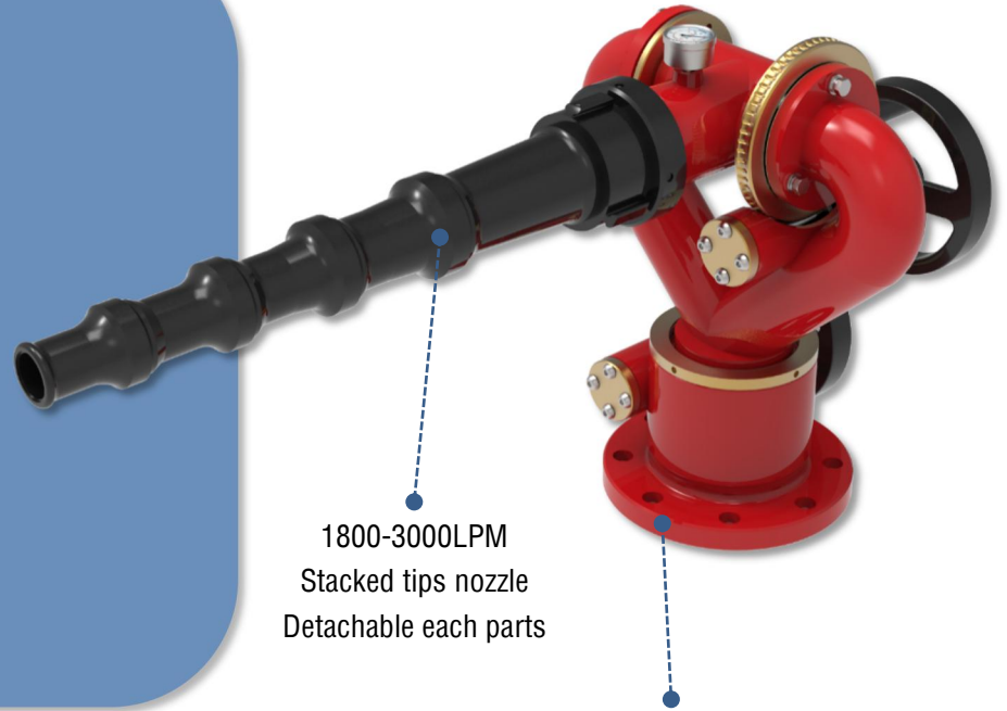
4" BS 4504 Flange is standard Thread inlet, other sizes & std. are available
